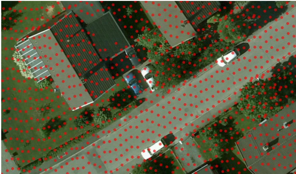
Figure 20. An example of the sparse nature of the laser strikes (all returns) and the actual laser footprint. The image also gives an example of points being absent over a roof.
