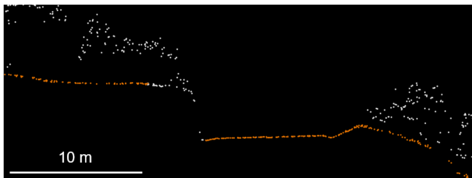
Figure 11. Rock wall by a road that has not been classified as ground, probably due to the steep incline. The profile is drawn according to the red line in the image below.
