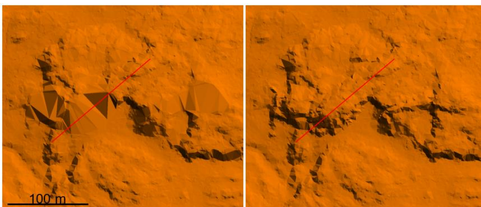
Figure 14. Shaded terrain image of the hill in the previous image. The left image shows how the terrain model looks after the automatic classification. The image to the right shows what the hill actually looks like, i.e. after reclassification.
