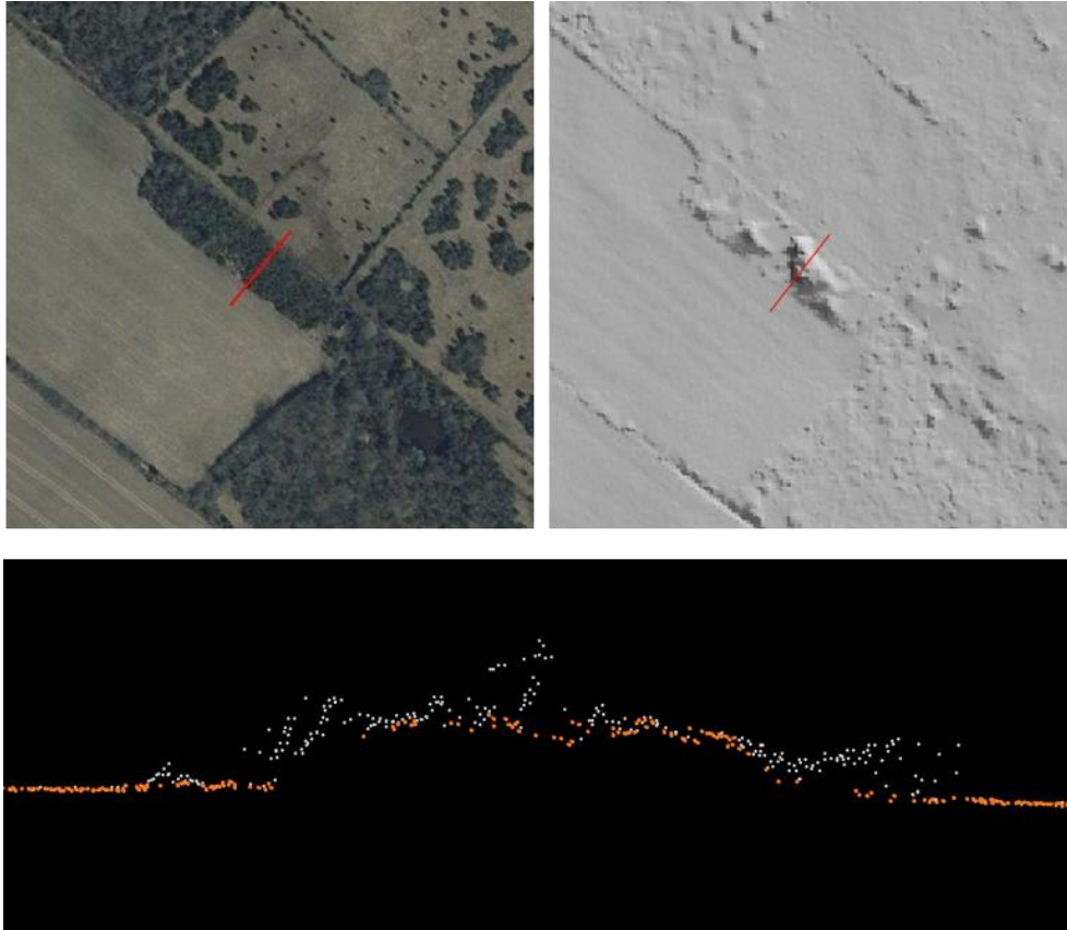
Figure 8. Dense low shrubbery, like juniper bushes on Öland's bare limestone, may register as land, i.e. small hills in the terrain model. As no laser pulses have penetrated the shrubbery and reached the ground, and as the bushes have a "smooth transition" to the ground, the bushes are perceived as ground by the algorithm in the automatic classification.
