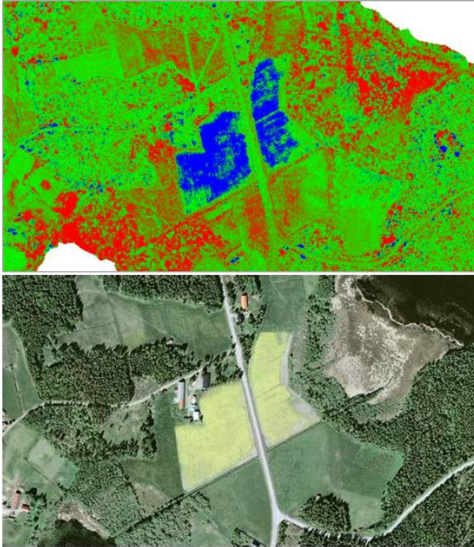
Figure 19. The upper image shows detail from a differential image between two scans conducted during different seasons. The lower image is an aerial photograph of the same section of terrain. The top right is an area of reeds, the middle is arable land, and the bottom left is reeds and other low vegetation. The differential image is green at 0 m difference and becomes totally red or blue at \pm 0.4 m difference in height.
