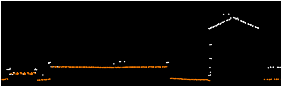
Figure 17. The roof of a parking structure has been classified as ground. The question is, however, where the ground should be.
