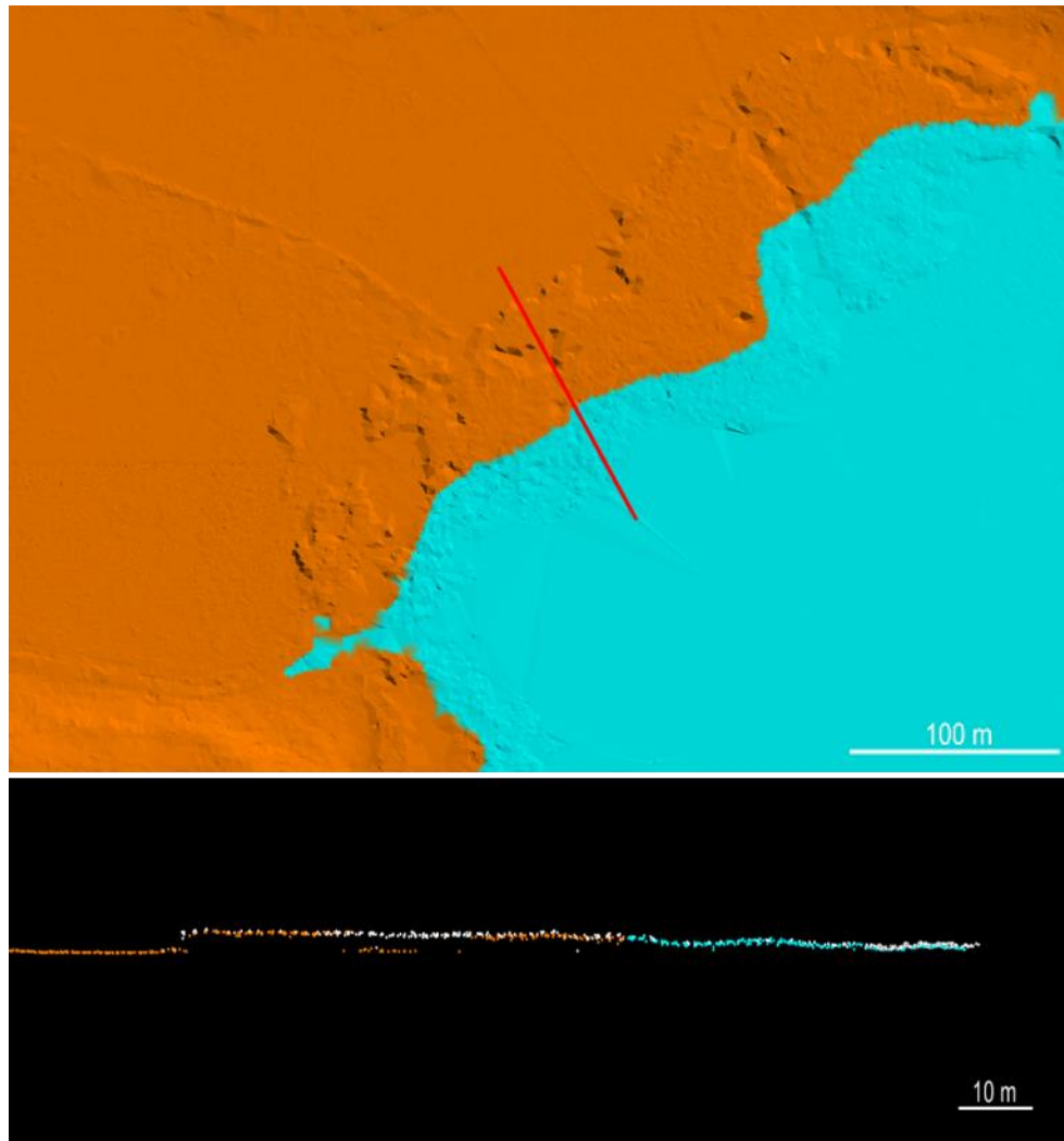
Figure 9. There is often a lack of points on the ground or water in dense reeds, and the reeds have been classified as ground in the automatic classification. Here, water is classified based on a water polygon in the GGD (classification level 2). The red line is the profile in the image beneath. The difference in elevation of a few metres between the ground and the reeds is clearly visible.
