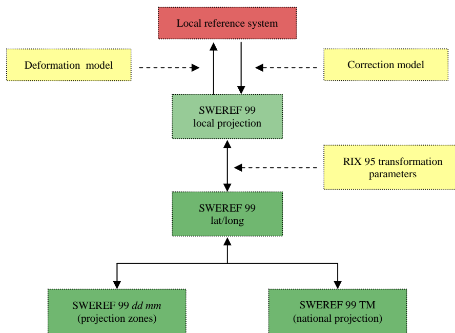
Figure 8: Transformation schedule for local reference systems to and from SWEREF 99.
