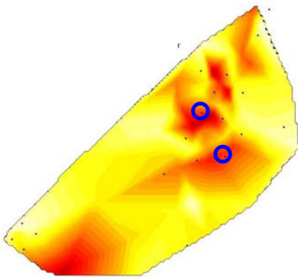
Figure 6: The variations of deformations of the local control network of Tranås, based on the residuals shown in figure 5. The deformations are weighted inversely to the square of the point distance. The two marked common control points were deviant, and finally excluded.
