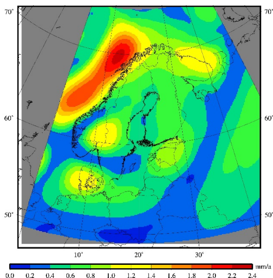
Figure 11.1: Uncertainty of the geophysical model NKG2016GIA_prel0306. Unit in mm/a.
